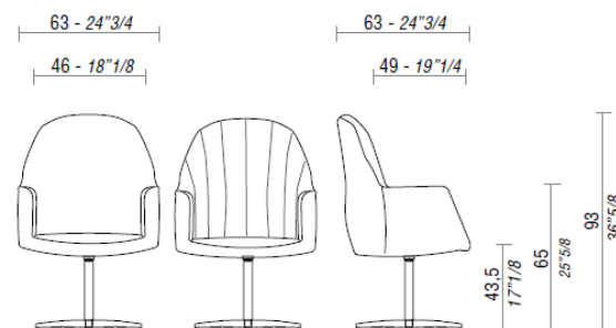
TULIP, POLTRONA BASE A CROCE CON SCHIENALE MEDIO TULIP, CHAIR WITH CROSS-SHAPED BASE AND MEDIUM BACKREST
